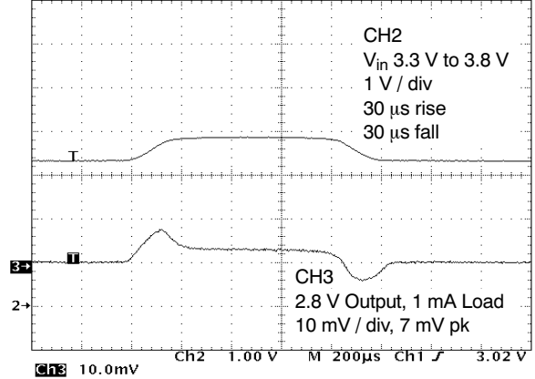
Figure 11. 2.8 V out vs. Line Transient
