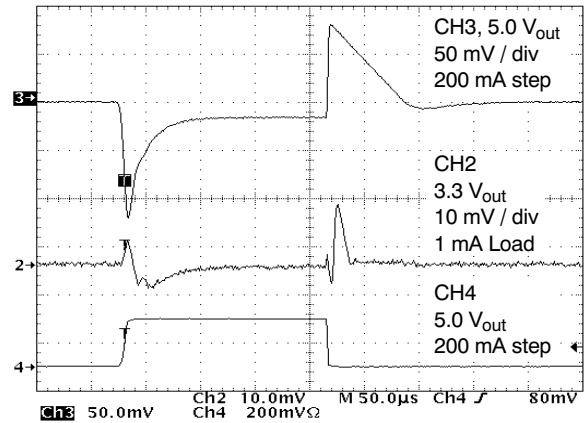
Figure 13. Load Transient on 5.0 V out and Effect on 3.3 V out for 200 mA Step
