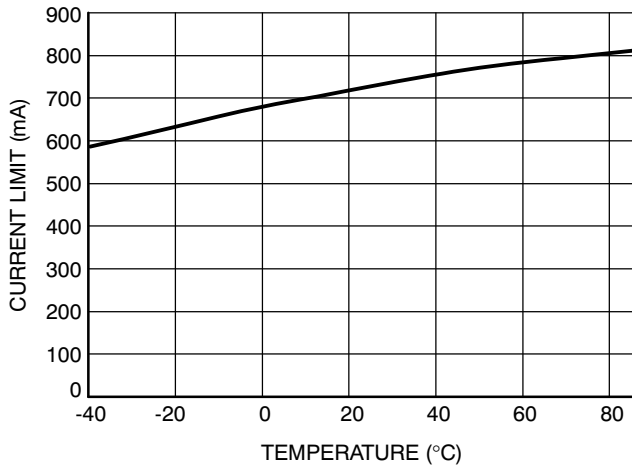
Figure 4. Current Limit vs. Temperature
