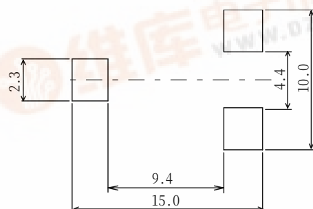
1-3. DIMENSION RECOMMENDED (mm)
