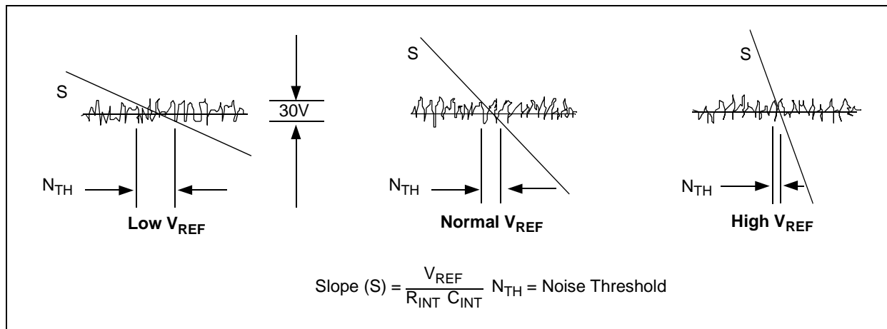
FIGURE 8-1: Noise Threshold.
