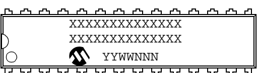
28-Lead PDIP (300 mil)
