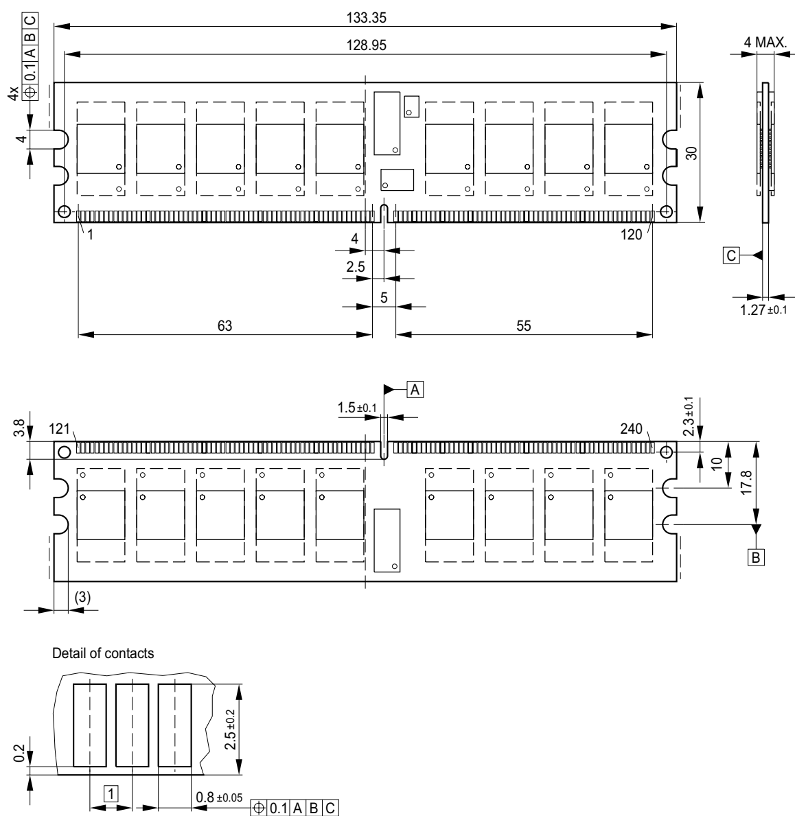
FIGURE 6 Package Outline Raw Card H L-DIM-240-13
