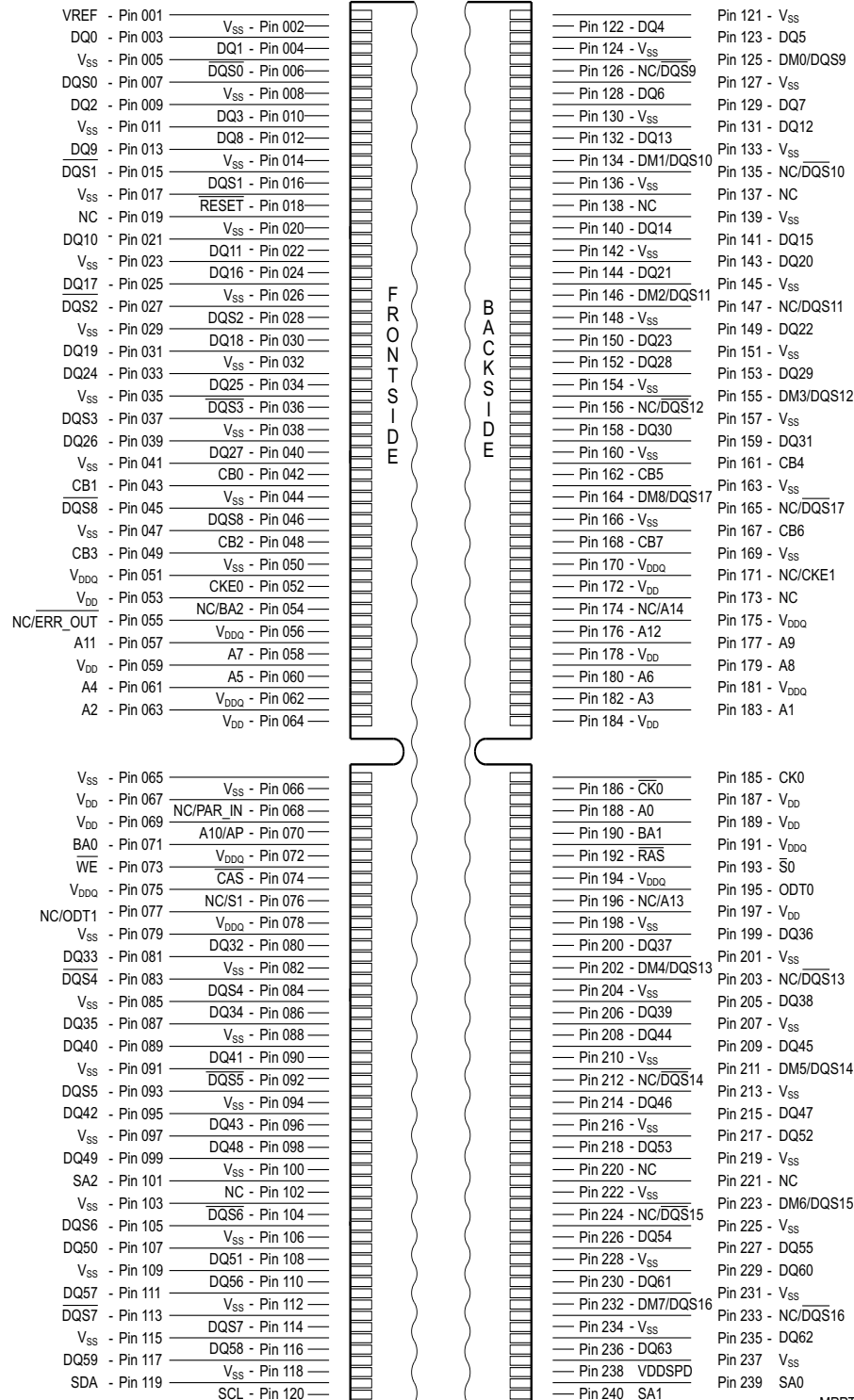
FIGURE 1 Pin Configuration for RDIMM (240 pins)
