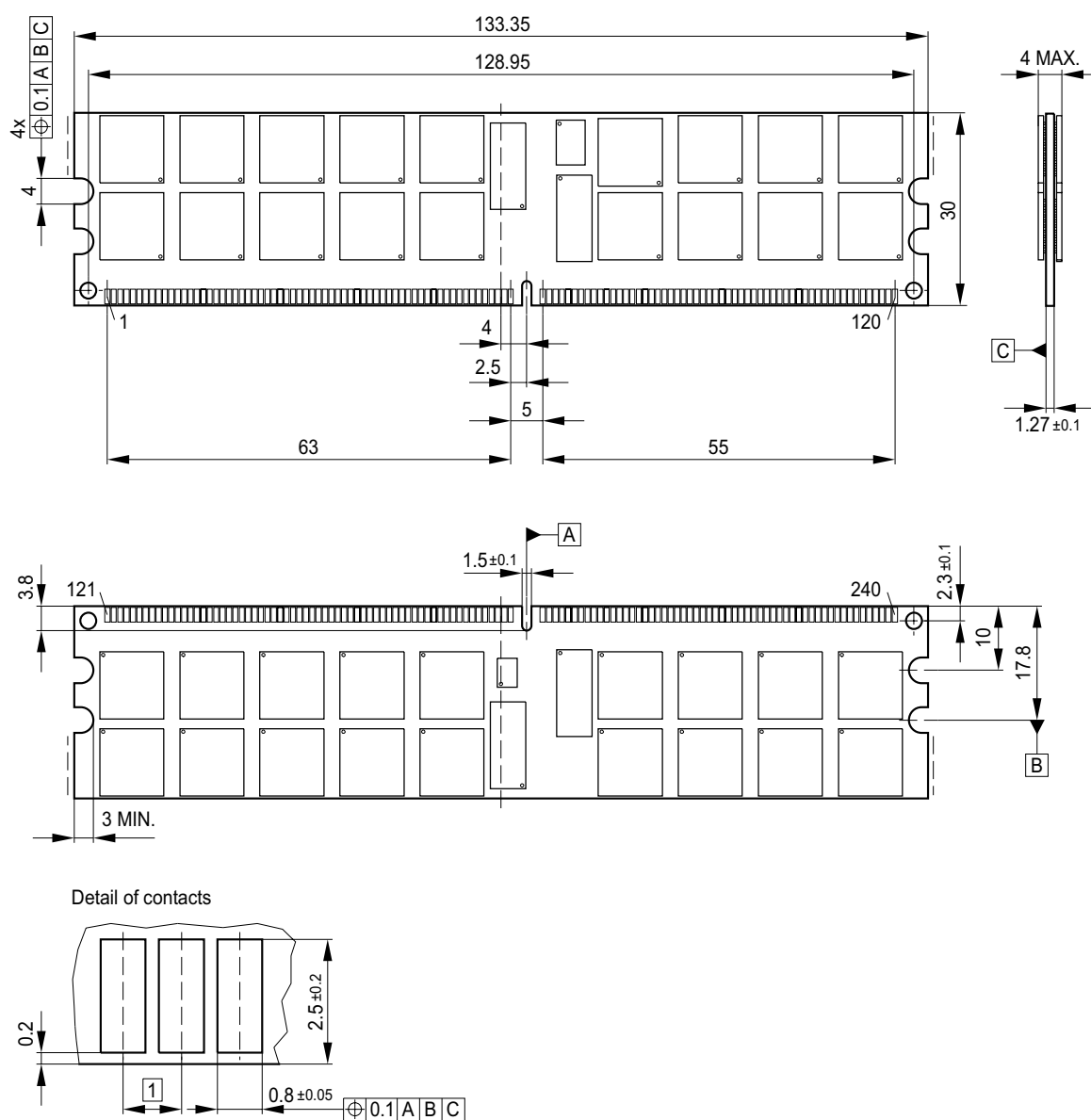
FIGURE 8 Package Outline Raw Card J L-DIM-240-20
