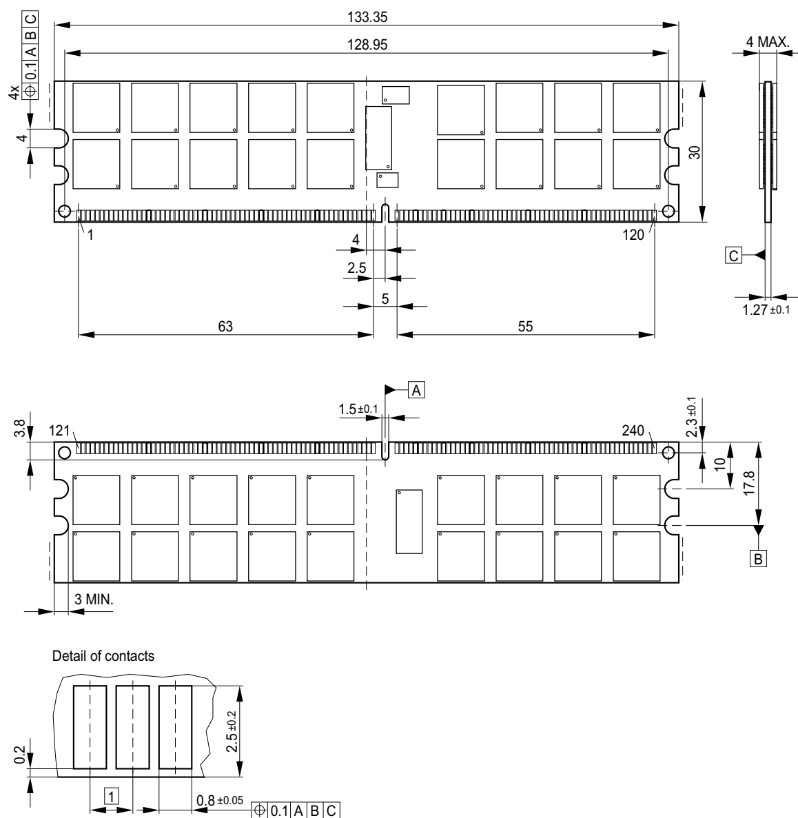
FIGURE 9 Package Outline Raw Card L L-DIM-240-48
