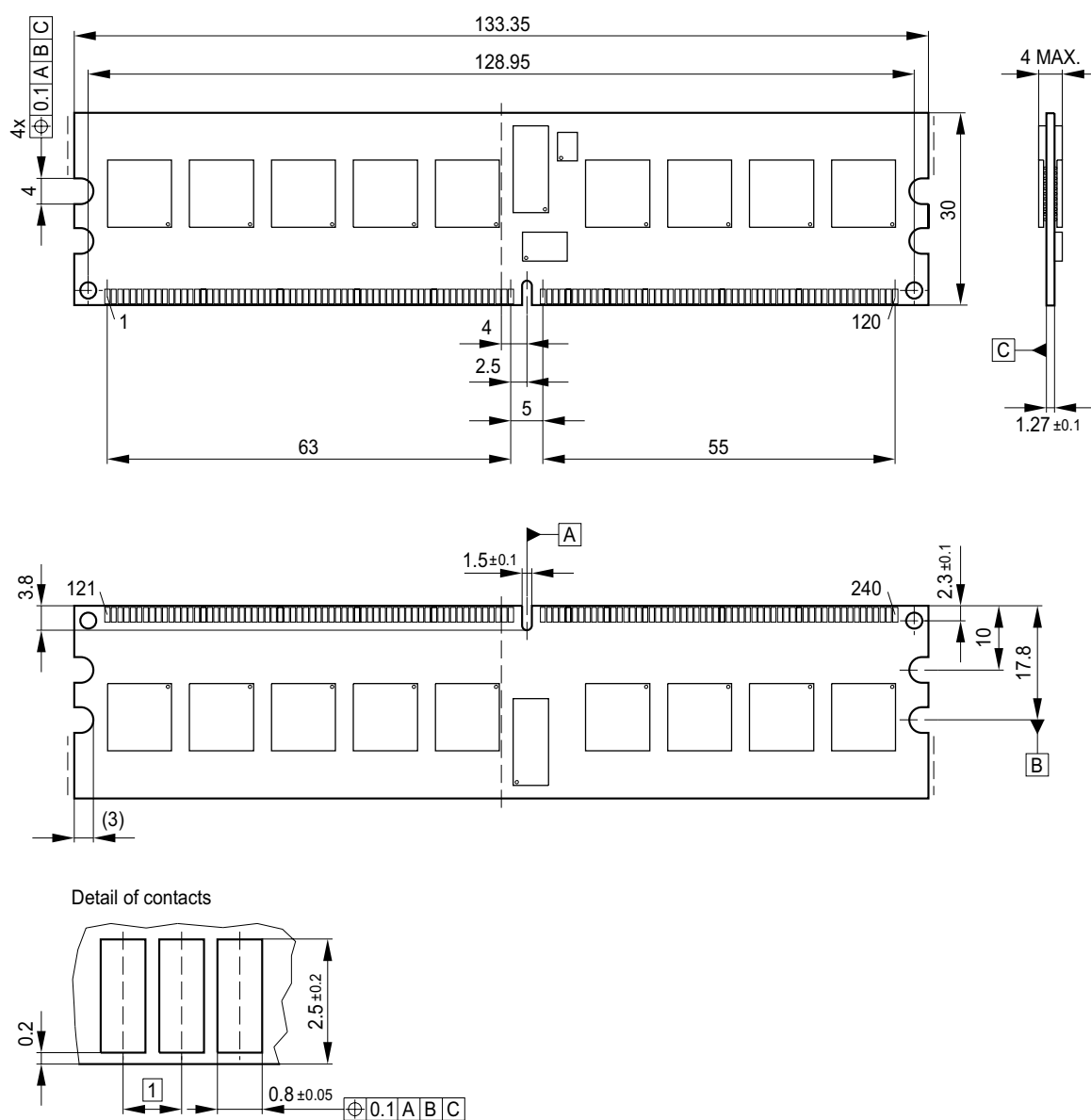
FIGURE 7 Package Outline Raw Card G L-DIM-240-12
