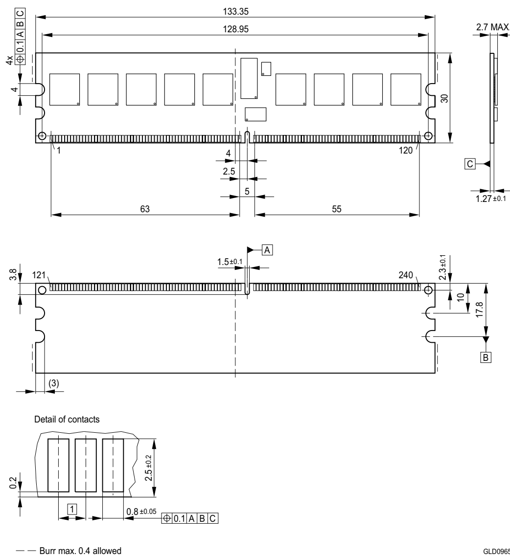
FIGURE 5 Package Outline Raw Card F L-DIM-240-11
