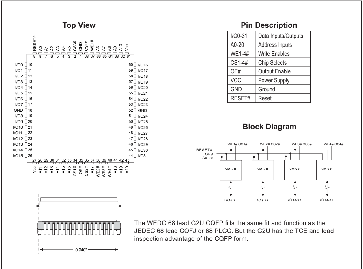
FIGURE 2 – PIN CONFIGURATION FOR WF2M32-XG2UX5
