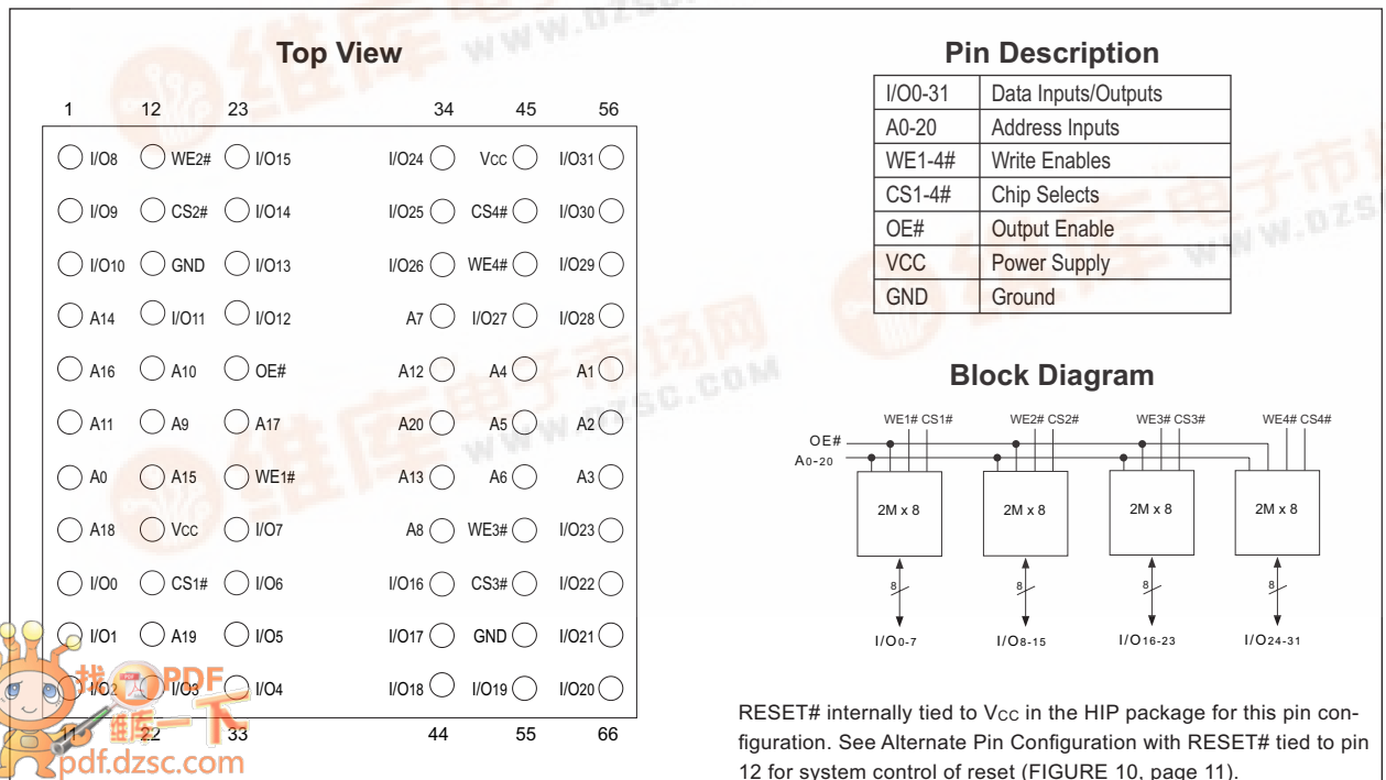
FIGURE 1 – PIN CONFIGURATION FOR WF2M32-XXH5
