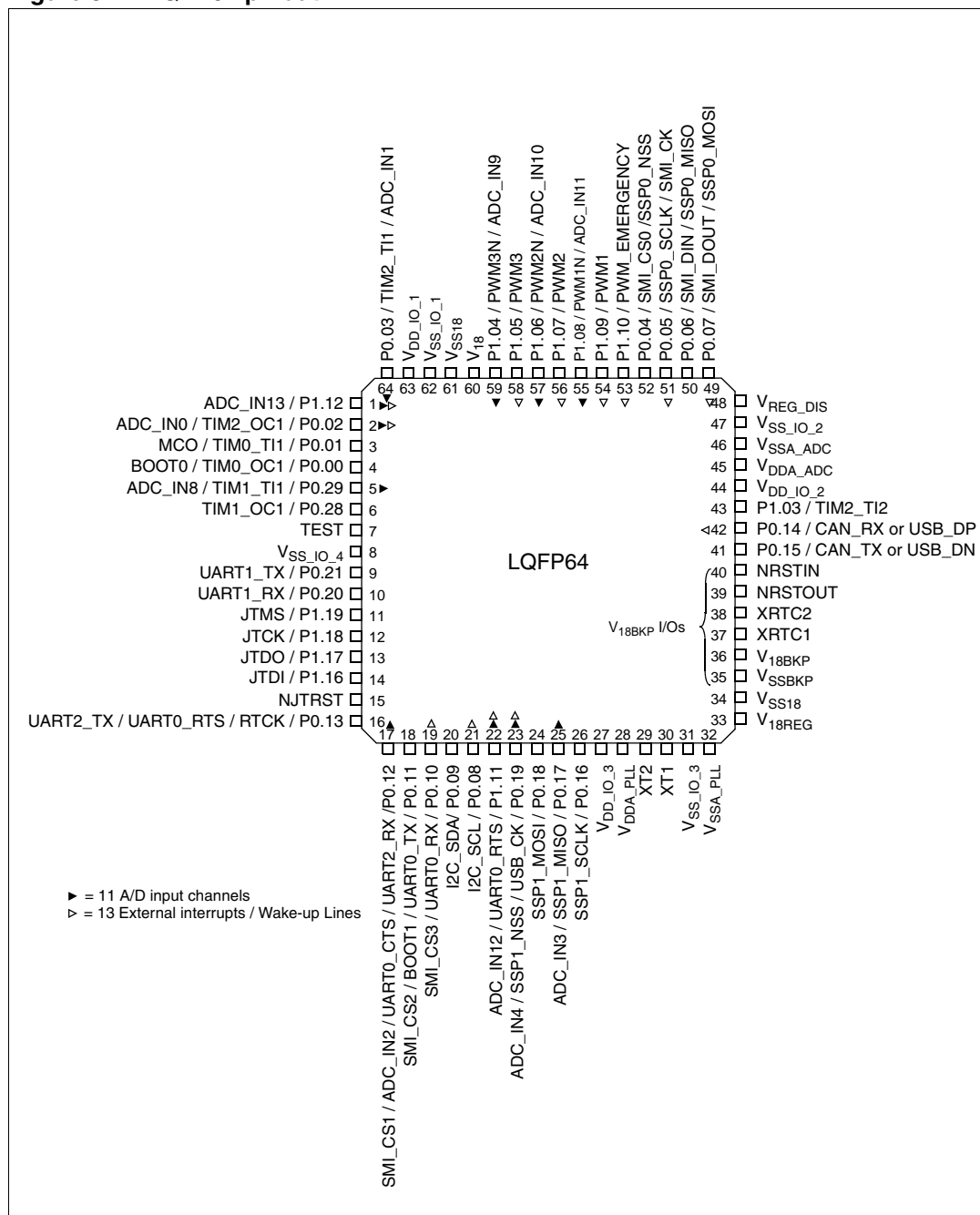
Figure 3. LQFP64 pinout
