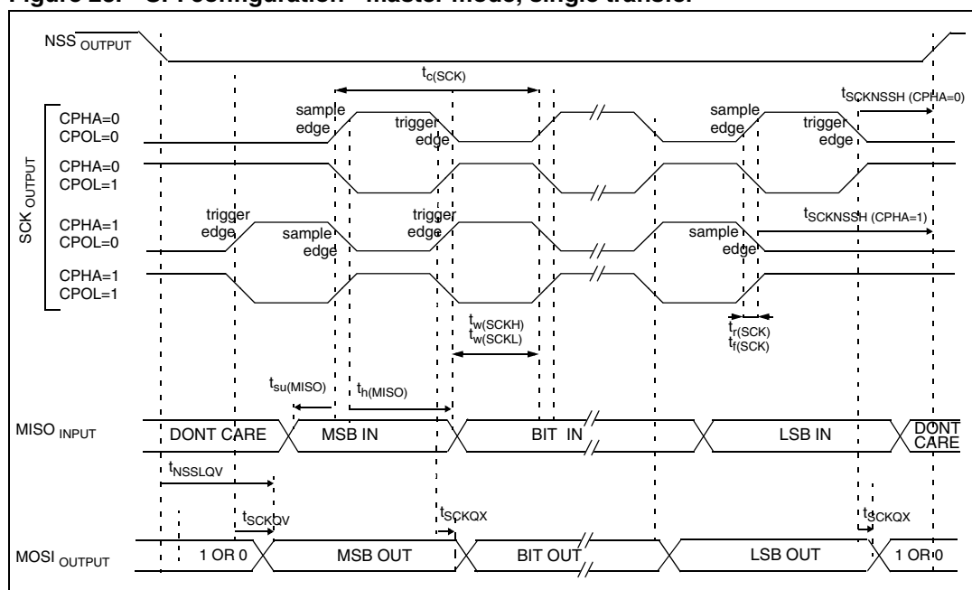
Figure 29. SPI configuration - master mode, continuous transfer, CPHA=0
