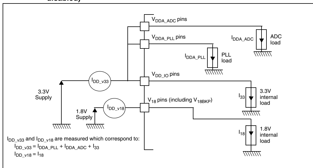
Figure 13. Power consumption measurements in power scheme 2 (regulators disabled)
