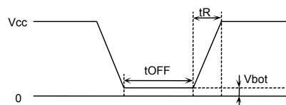
Fig.62 Rise waveform
