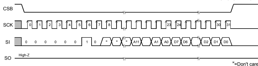
Fig.38 Write command (BR25H080/160/320-W) *=Don't care
