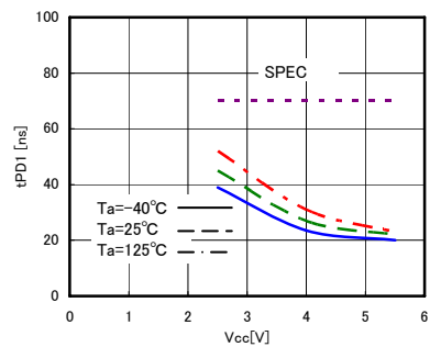
Fig.23 Data output delay time t_{PD1}(CL=100\text{pF})
