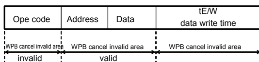
Fig.45 WPB valid timing (WRITE)
