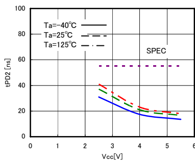
Fig.24 Data output delay time t_{PD2}(CL=30\text{pF})
