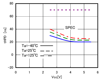
Fig.29 Time from HOLDB to output change t_{HPD}
