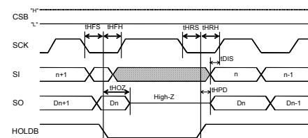
Fig.5 HOLD timing
