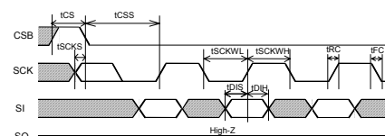
Fig.3 Input timing
