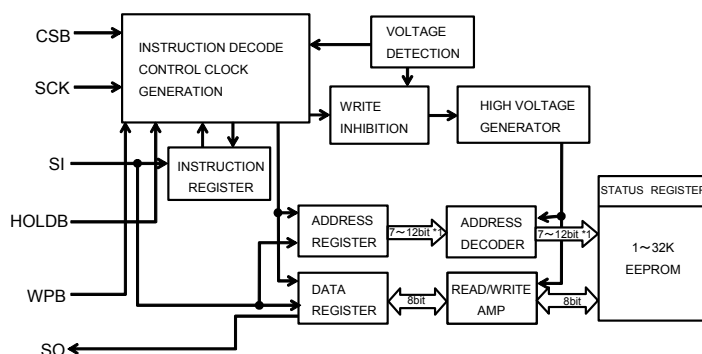
Fig.1 Block diagram
