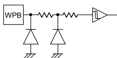
Fig.60 WPB input equivalent circuit
