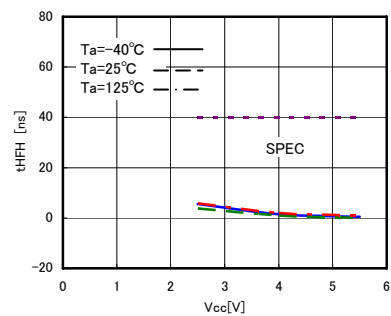
Fig.26 HOLDB setting hold time t_{HFH}
