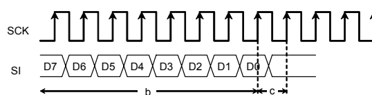
Fig.48 WRITE cancel valid timing
