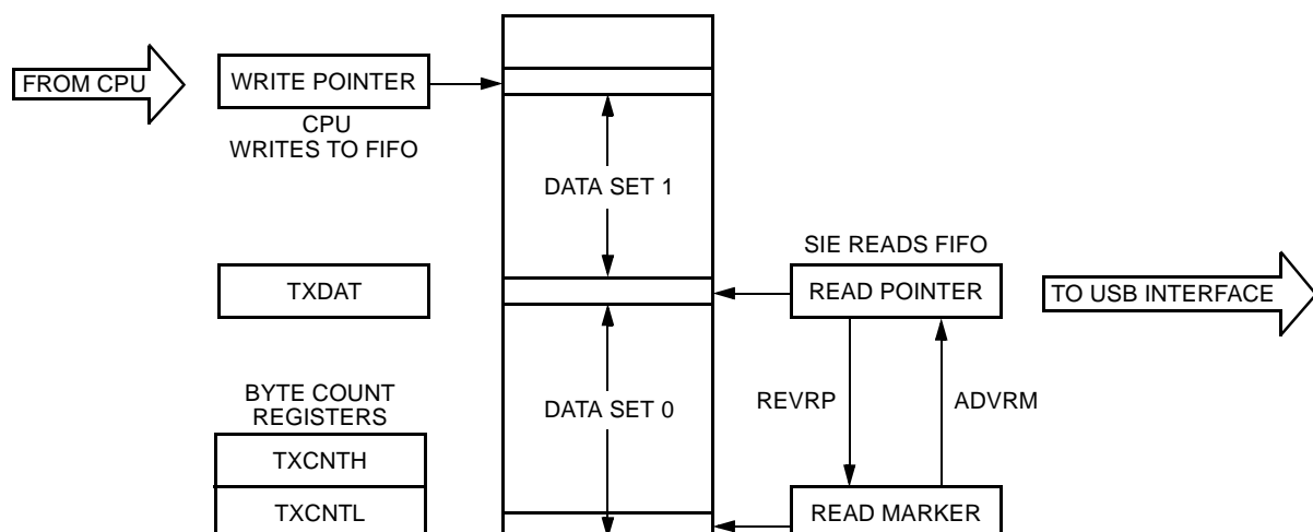
Figure 2. Transmit FIFO
