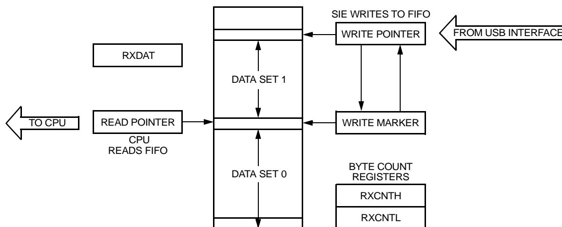
Figure 3. Receive FIFO
