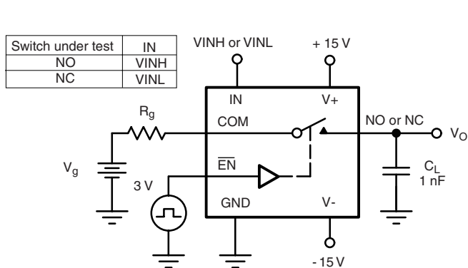
Figure 3. Charge Injection
