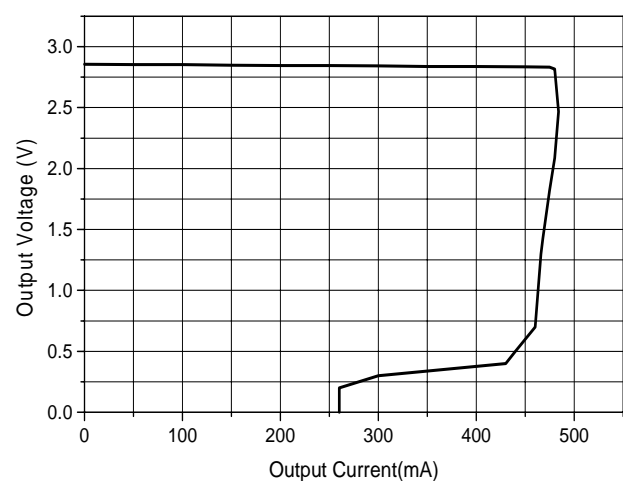
Overcurrent Protection
