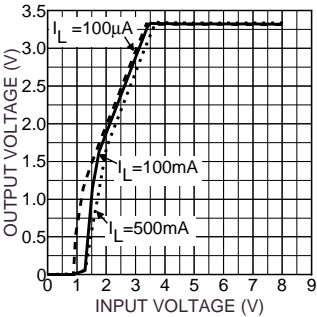
Dropout Characteristics
