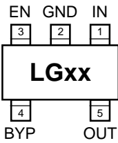
MIC5219-x.xBM5 SOT-23-5 Fixed Voltages
