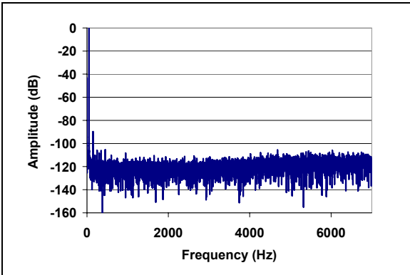
FIGURE 2-28: Frequency Spectrum, 50 Hz Input Signal.
