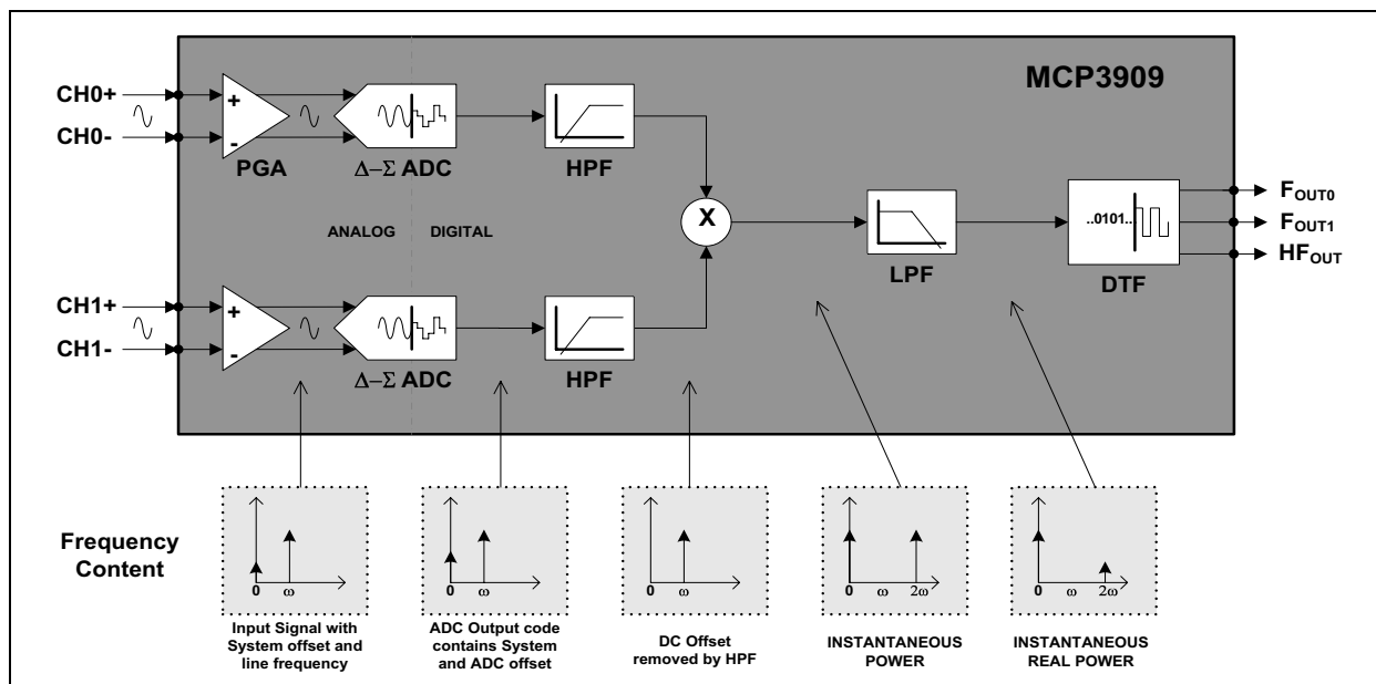
FIGURE 4-1: Active Power Signal Flow with Frequency Contents.
