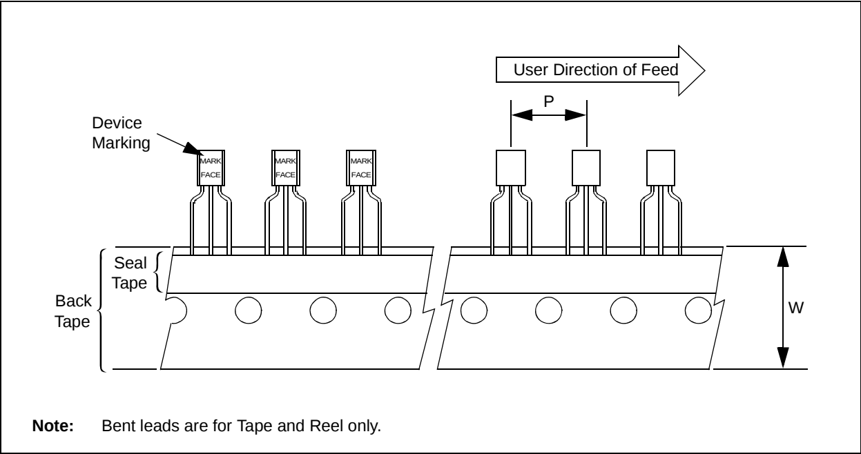
FIGURE 5-3: TO-92 DEVICES
