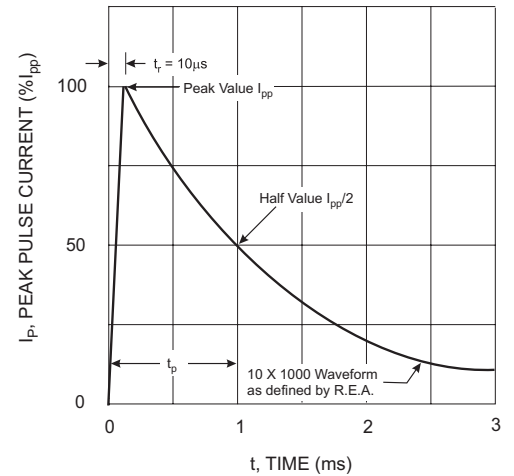
Fig. 4 Pulse Waveform
