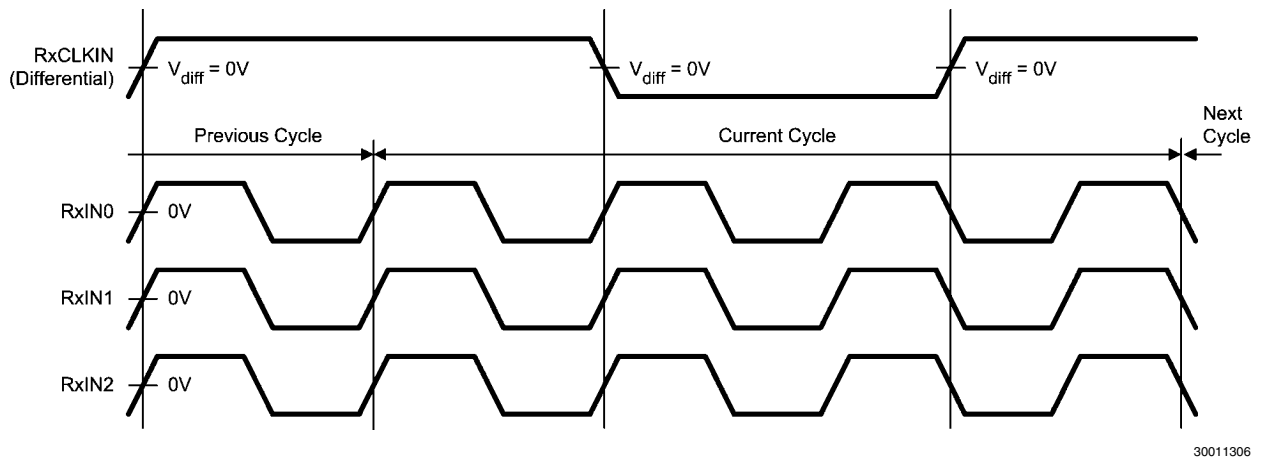
FIGURE 3. LVDS Input Checkerboard Pattern
