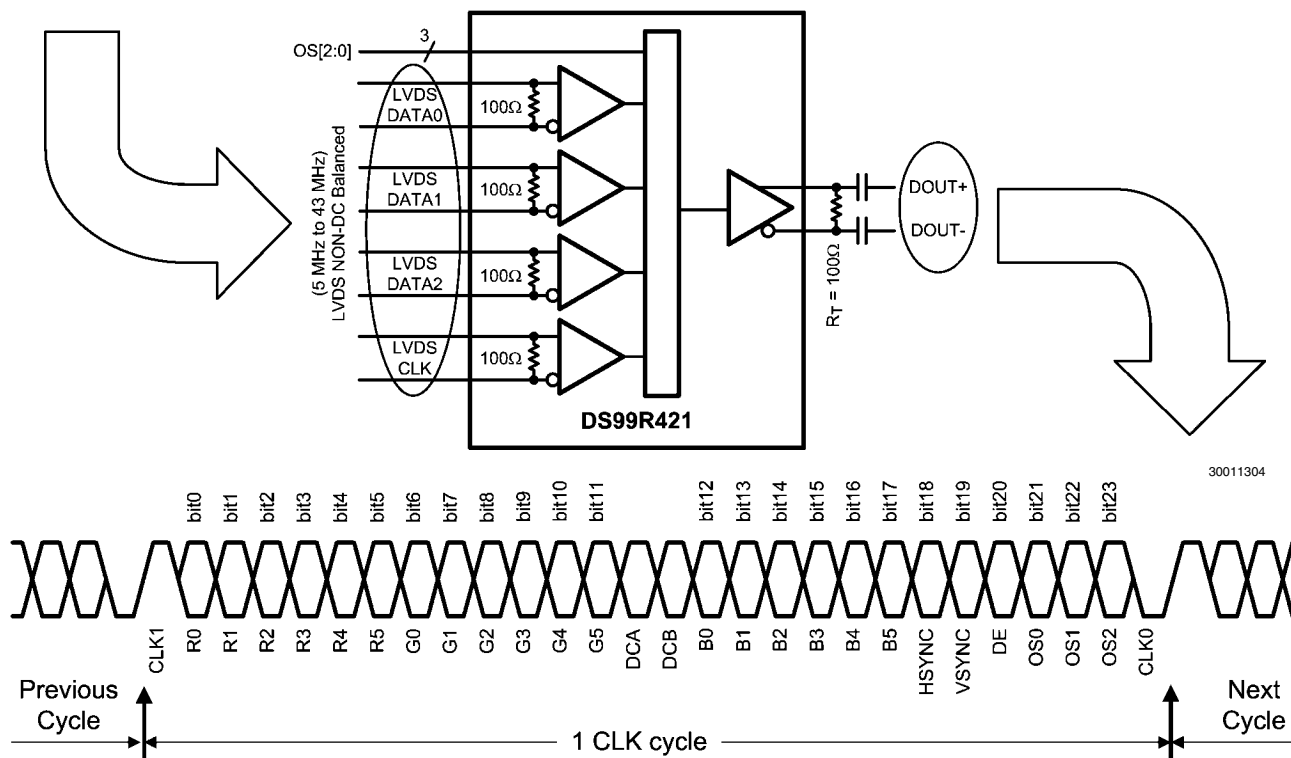
FPD-Link LVDS Input Mapping (3 LVDS Data + 1 LVDS Clock)
