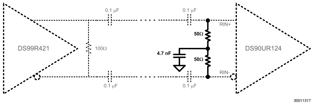
FIGURE 14. Receiver Termination Option 2
