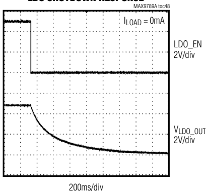
LDO SHUTDOWN RESPONSE
