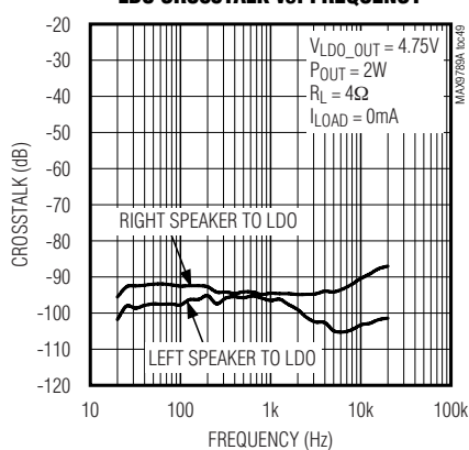
LDO CROSSTALK vs. FREQUENCY
