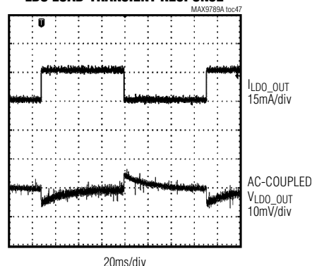
LDO LOAD-TRANSIENT RESPONSE
