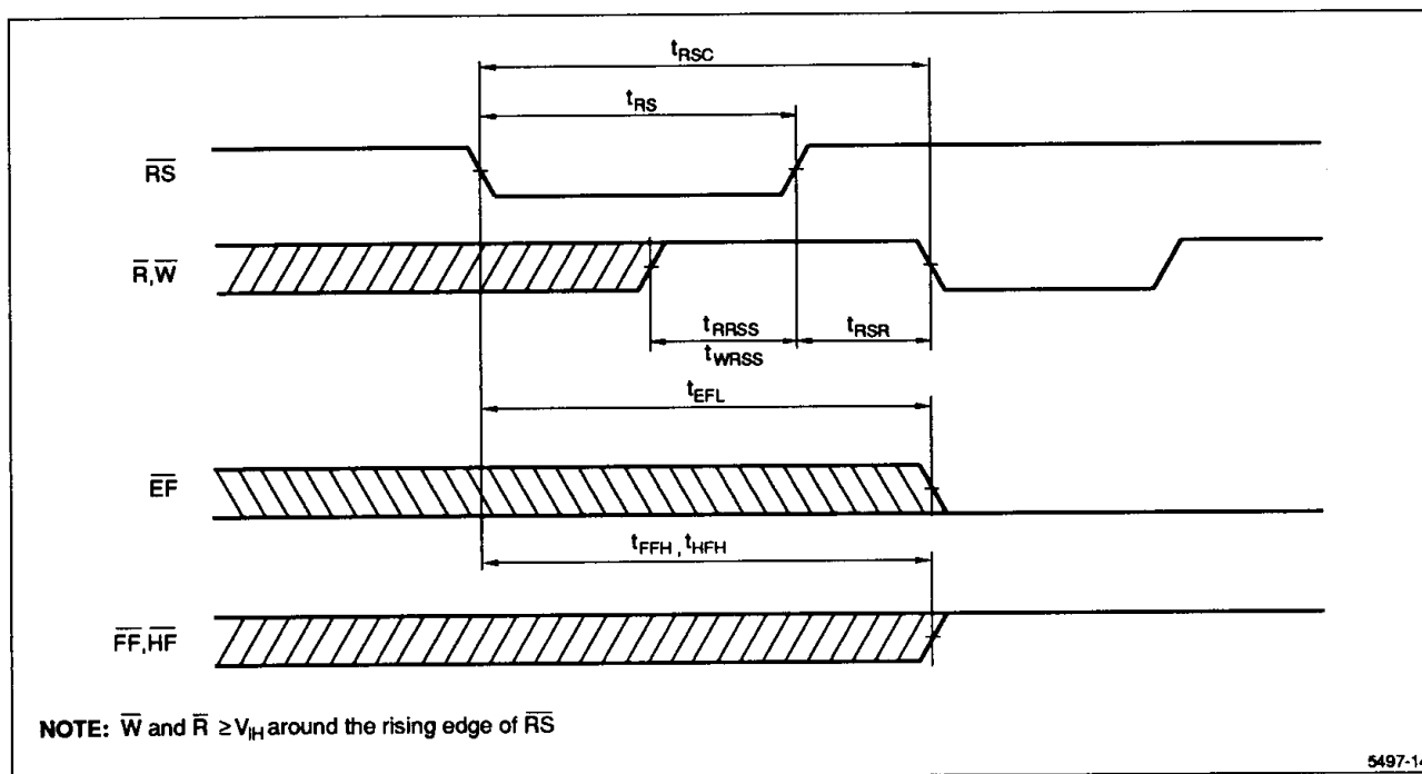
Figure 5. Reset Timing
