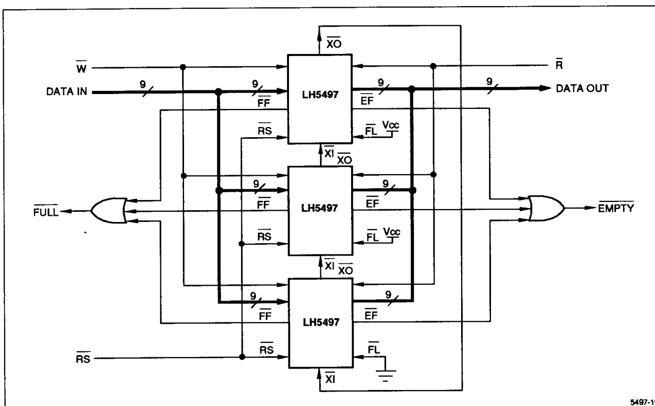
Figure 19. FIFO Depth Expansion (3072 \times 9)
