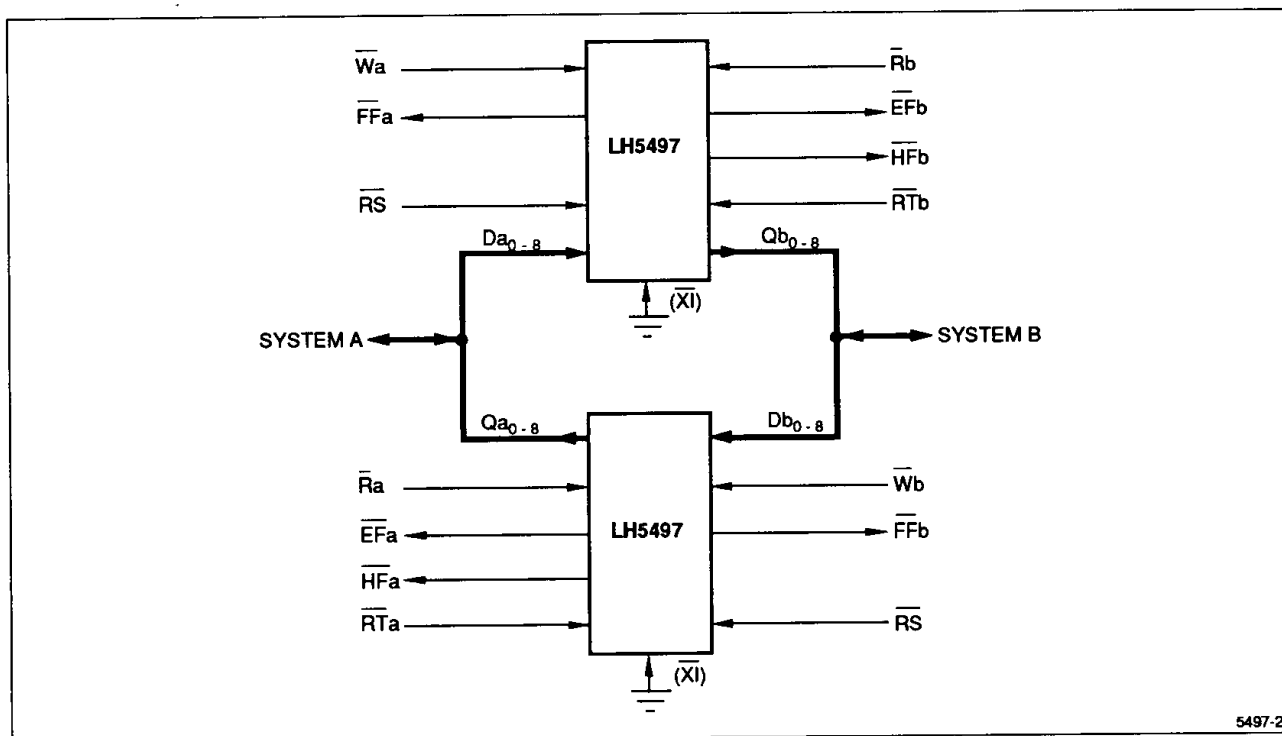
Figure 21. Bidirectional FIFO
