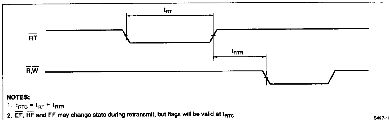
Figure 14. Retransmit Timing
