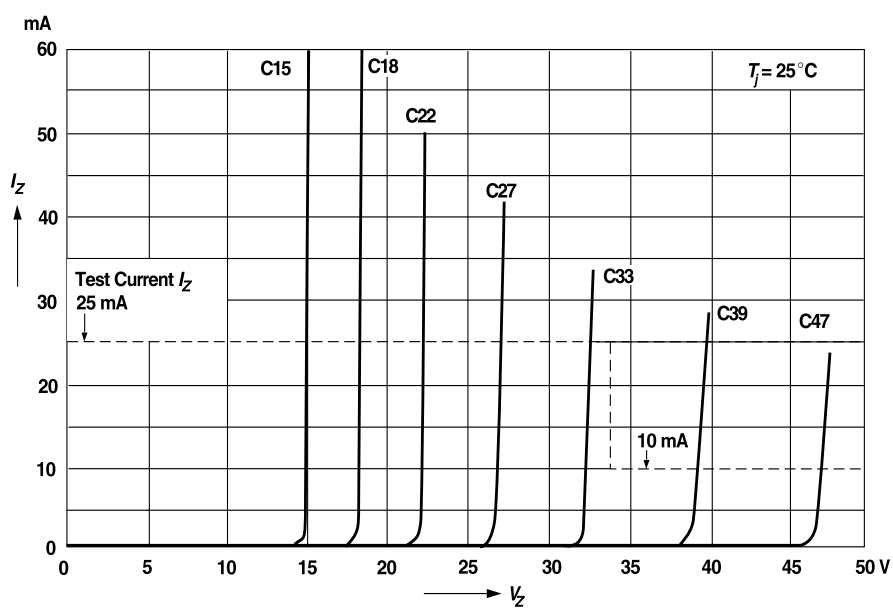
Figure 7. Breakdown Characteristics
