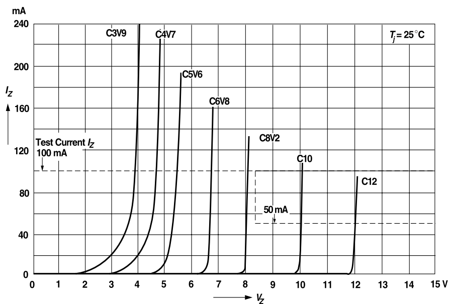
Figure 6. Breakdown Characteristics
