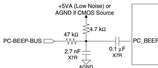
Figure 15. PC_BEEP Input
