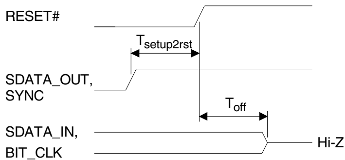
Figure 6. Test Mode
