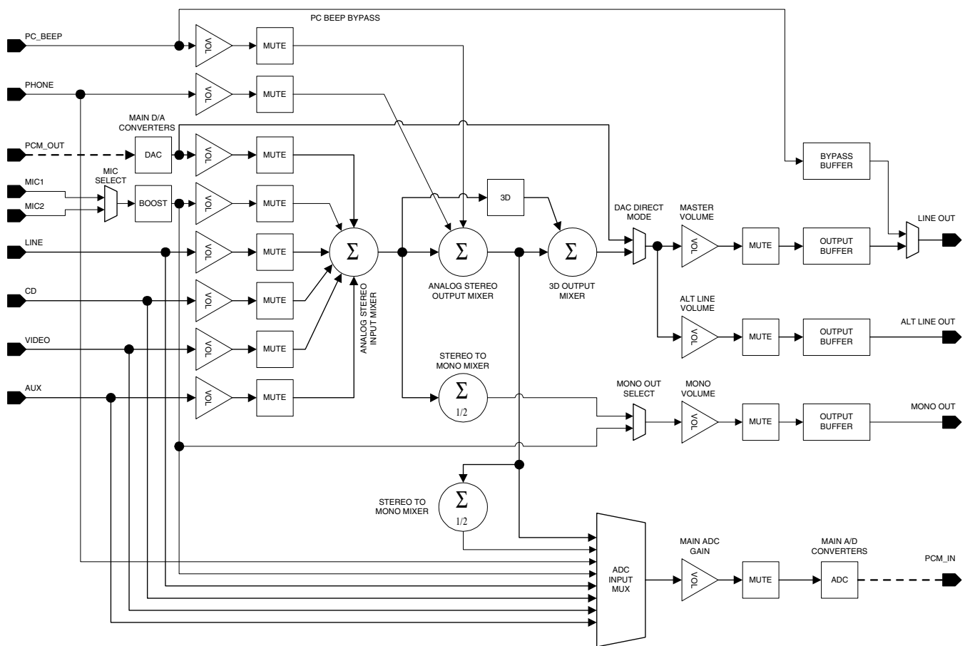
Figure 8. Mixer Diagram
