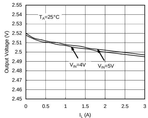
G9966-25 Output Voltage vs. I_L
