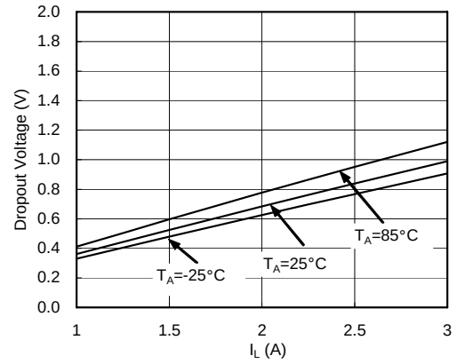
G9966-18 Dropout Voltage vs. I_L
