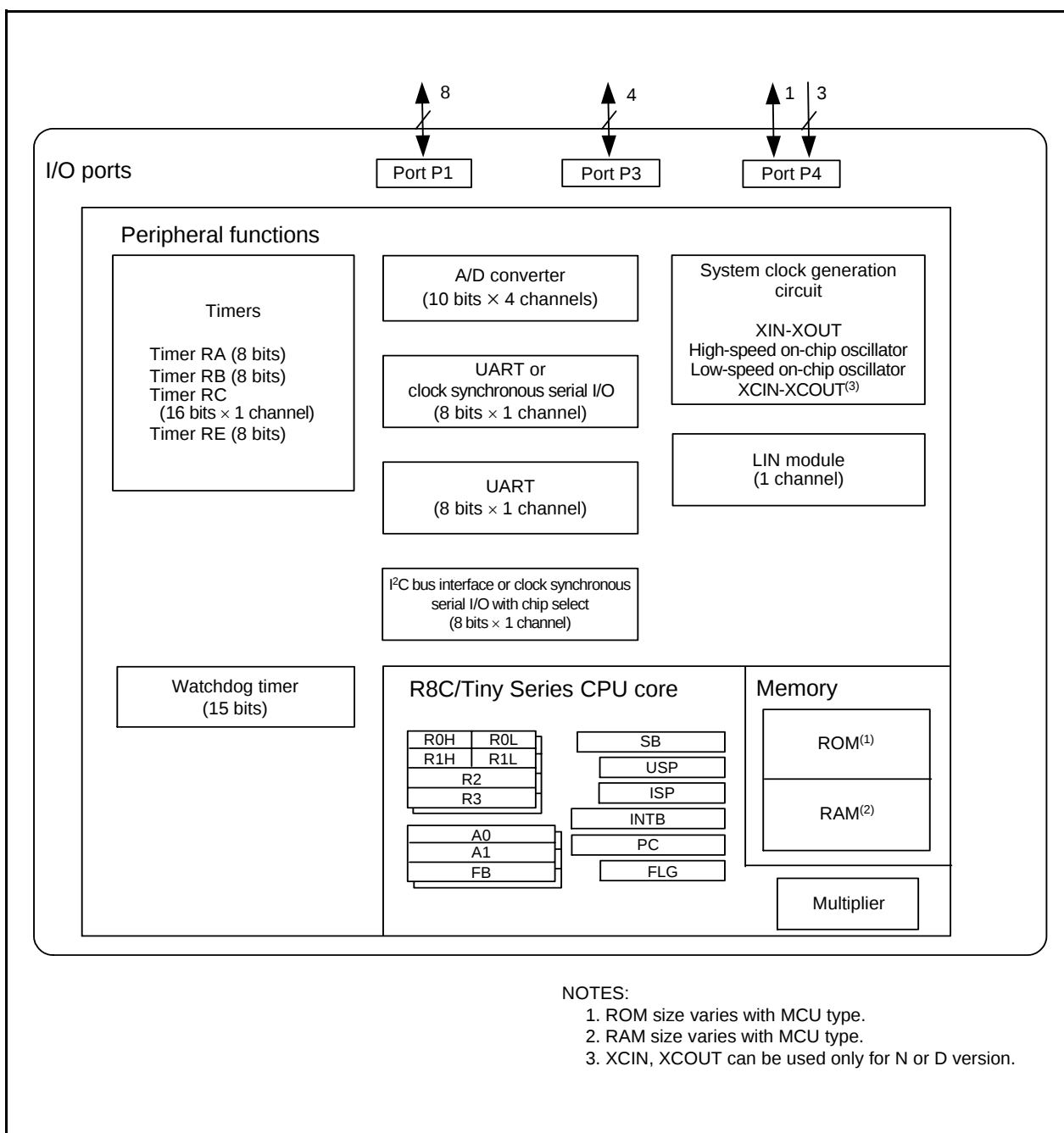
Figure 1.1 Block Diagram
