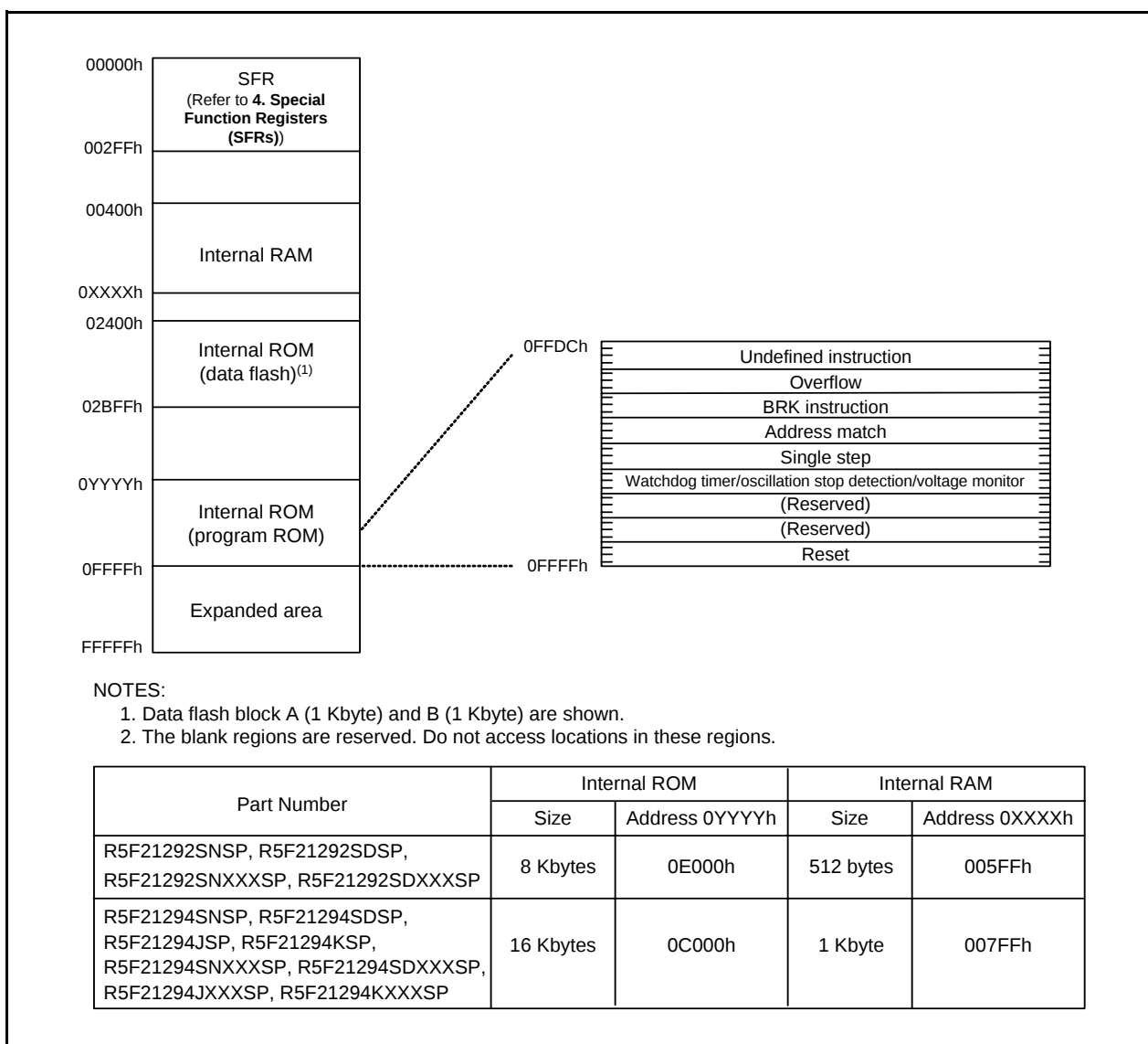
Figure 3.2 Memory Map of R8C/29 Group
