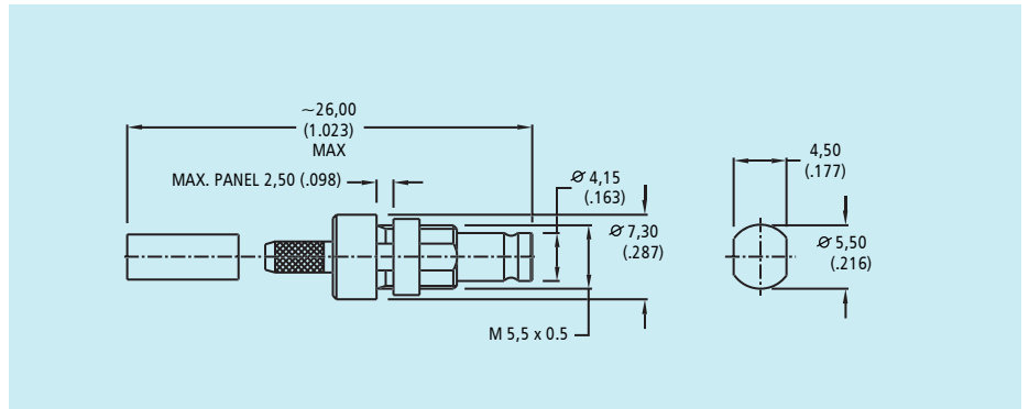
Assembly Instructions BBAI - 1281 - page 29
