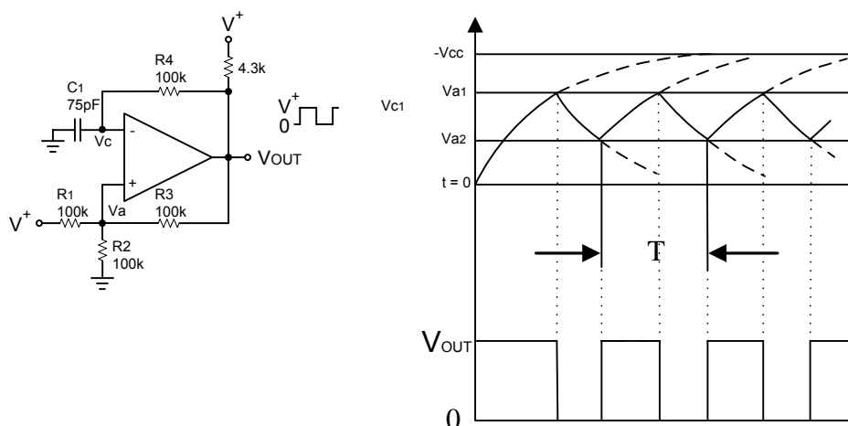
Squarewave Oscillator
