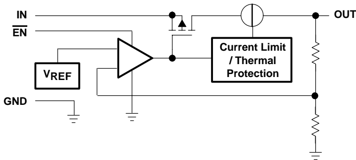
TPS76912/15/18/25/27/28/30/33/50-Q1
