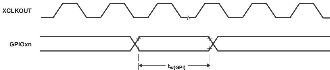
Figure 6-11. General-Purpose Input Timing
