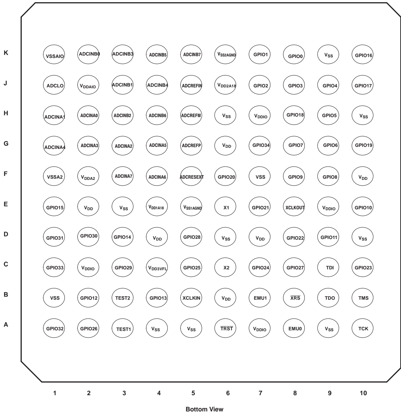
Figure 2-5. TMS320F2809, TMS320F2808, TMS320F2806, TMS320F2802, TMS320F2801, TMS320F28016, TMS320F28015, TMS320C2802, TMS320C2801 100-Ball GGM and ZGM MicroStar™ (Bottom View)
