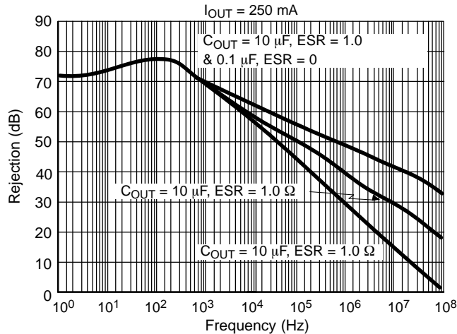
Figure 10. Ripple Rejection
