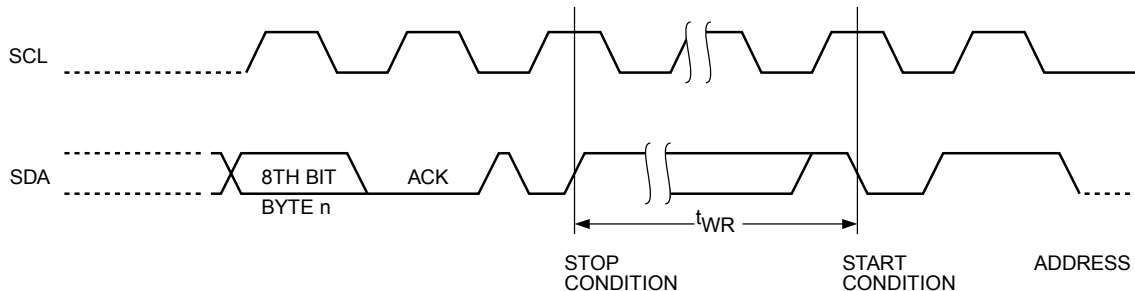
Figure 3. Start/Stop Timing
