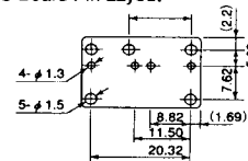
PC Board Pin Layout
