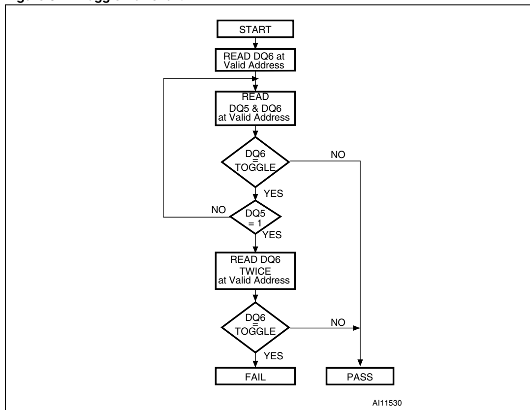
Figure 6. Toggle flowchart
