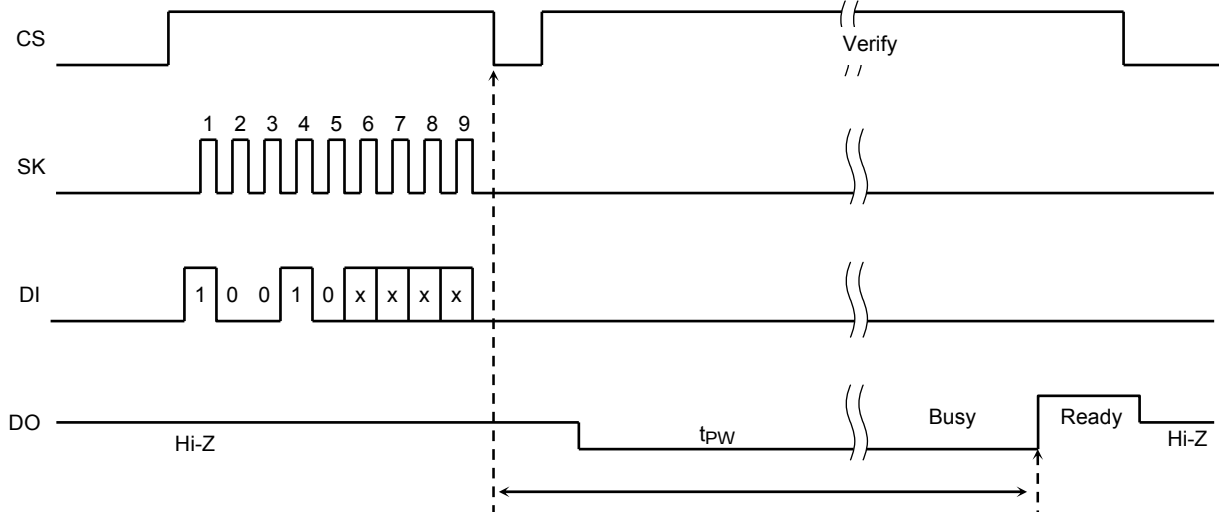
Figure 9. Erase Timing Diagram (TC9WMC1)
