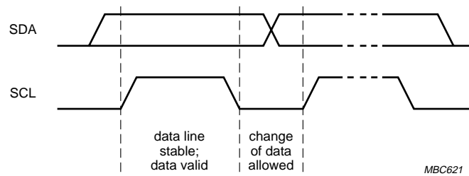
Fig.21 Bit transfer.
