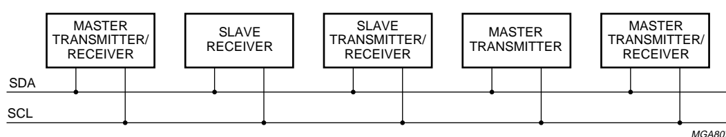
Fig.20 System configuration.
