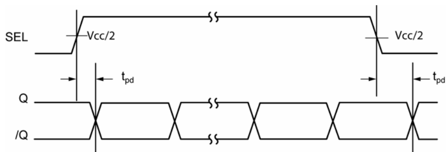
Figure 1c. SEL-to-Q Delay
