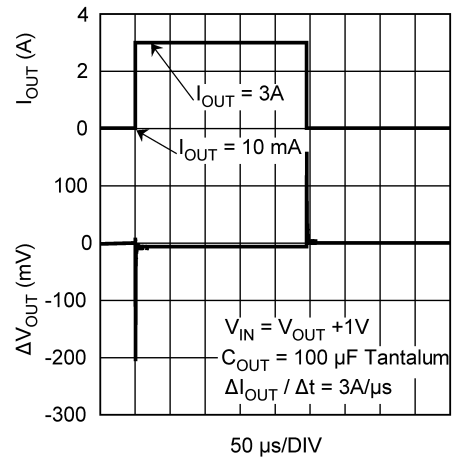
Load Transient Response, C_{OUT} = 100\text{ }\mu\text{F} Tantalum
