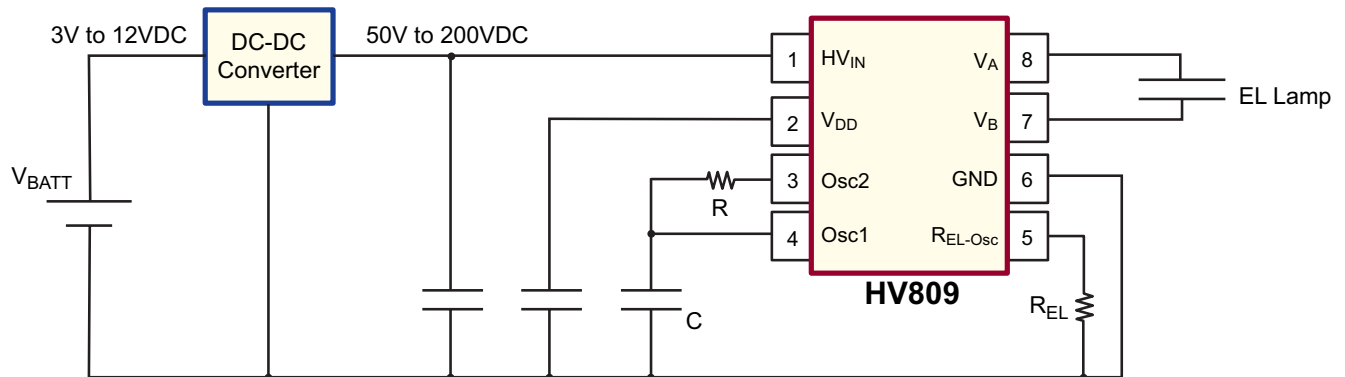
Figure 2. Pulsing EL Lamp
