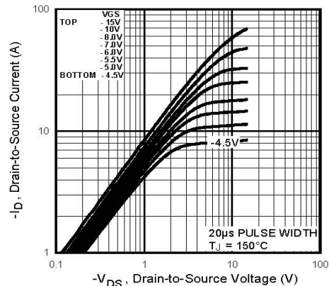
Fig 13. Typical Output Characteristics, T_J = 150^\circ\text{C}
