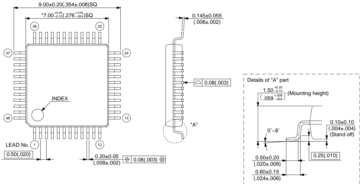
48-pin Plastic LQFP (FPT-48P-M05)
