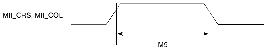
Figure 76. MII Async Inputs Timing Diagram
