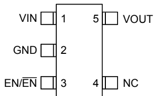
SOT-23-5/SC-70-5 (R-Type)
