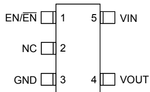
SOT-23-5/SC-70-5
