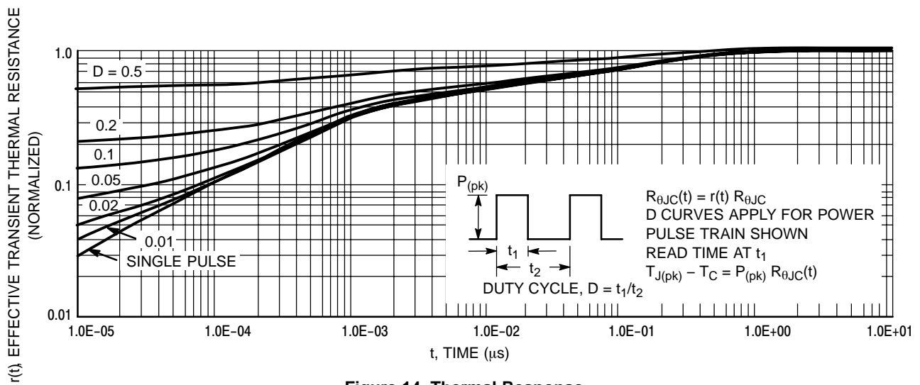
Figure 14. Thermal Response
