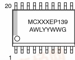
SOIC-20 DW SUFFIX CASE 751D
