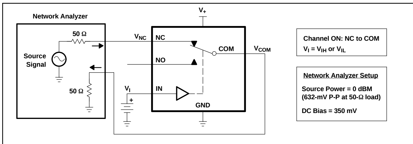
Figure 17. Bandwidth (BW)
