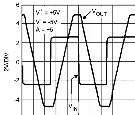
Overload Recovery Waveform
