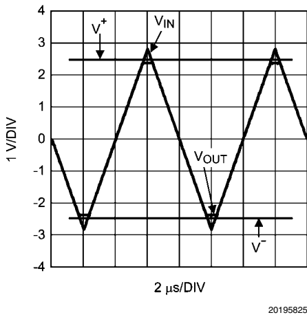
FIGURE 1. Input and Output Shown with CMVR Exceeded
