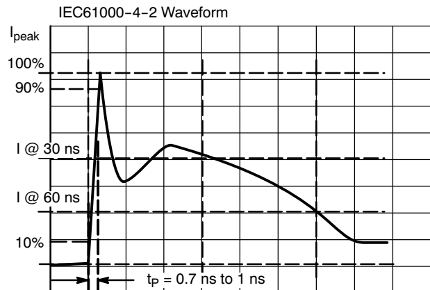
Figure 3. IEC61000-4-2 Spec
