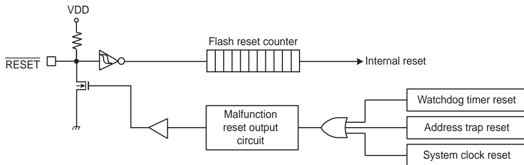
Figure 2-16 Reset Circuit
