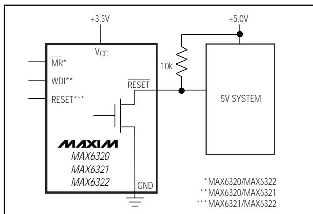
Figure 6. MAX6320P/MAX6321HP/MAX6322HP Open-Drain \overline{RESET} Output Allows Use with Multiple Supplies
