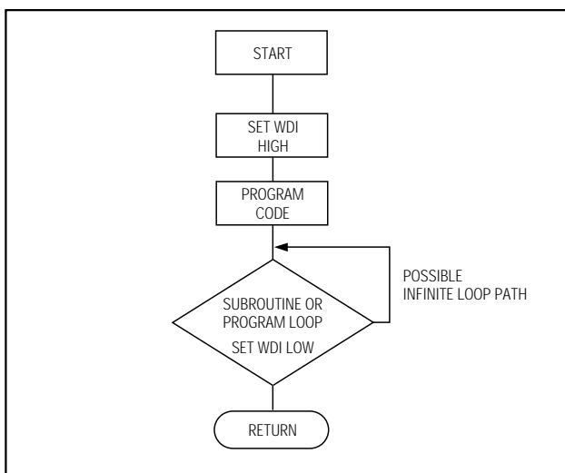
Figure 10. Watchdog Flow Diagram
