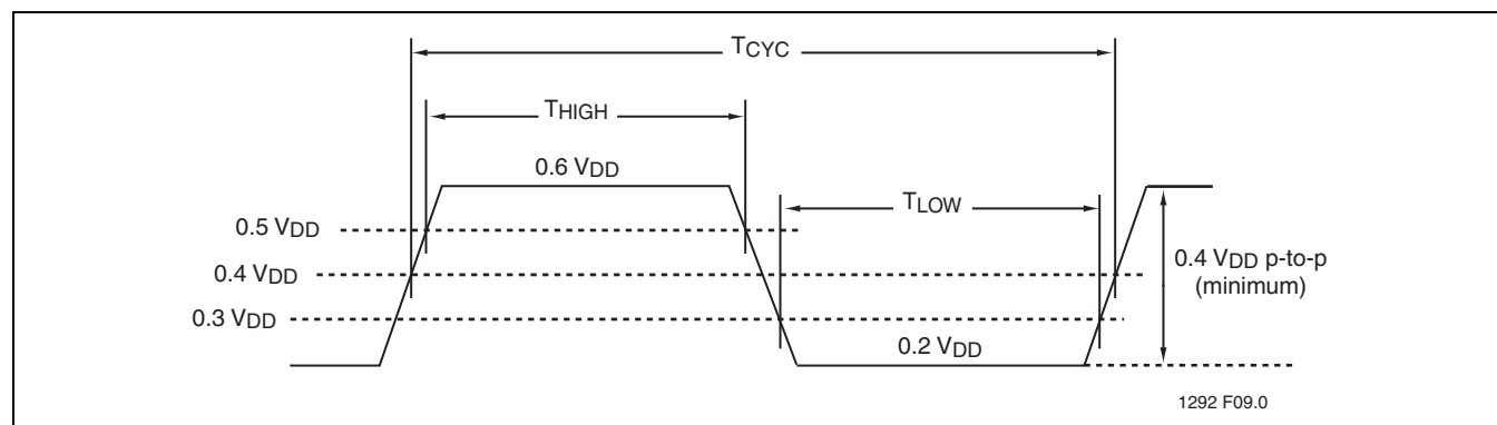
FIGURE 9: LCLK WAVEFORM (LPC MODE)
