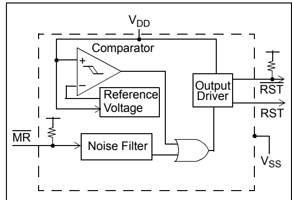
FIGURE 4-12: MCP1322 Block Diagram.
