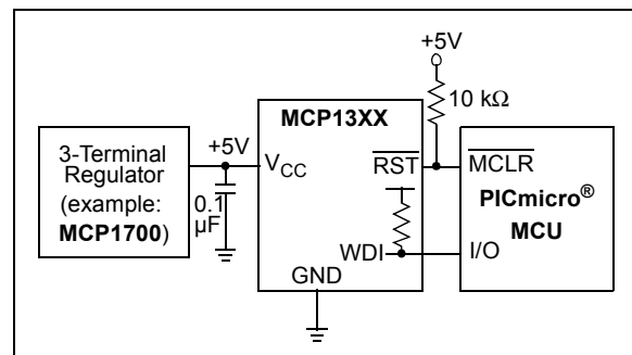
FIGURE 4-19: Watchdog Timer.
