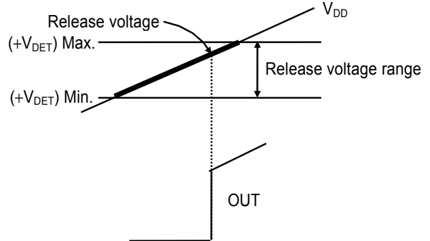
Figure 22 Release Voltage (CMOS Output Products)
