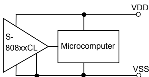
Figure 27 Reset Circuit Example (S-808xxCL)
