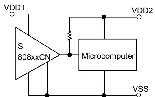
Figure 28 Reset Circuit Example (S-808xxCN)
