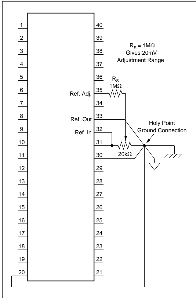
FIGURE 7. V_{REF} Adjust.
