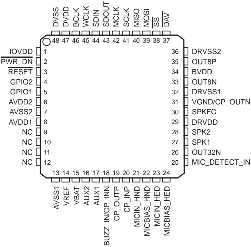
QFN PACKAGE (TOP VIEW)
